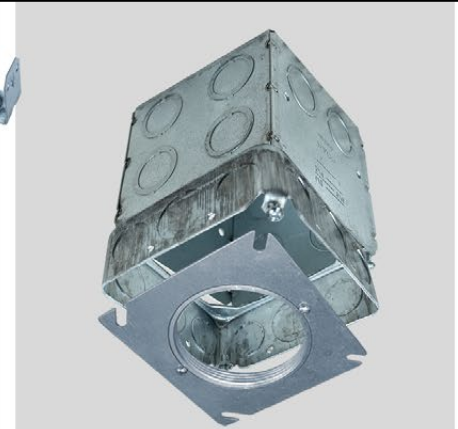
Step 2- Attach J-Box Mounting Hardware with threaded ring inserted (ring up) into J-BOX using two screws.
