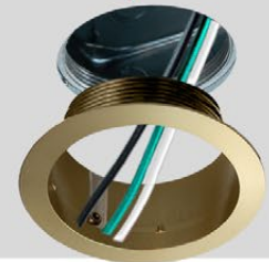
Step 5- Pull power supply and control wires (if required) through ceiling aperture and through the flanged receiver before threading receiver into J-box mounting hardware. Thread until flange receiver is tight to ceiling.
