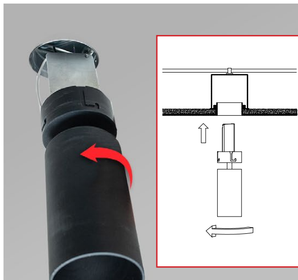
Step 7- Align fixture j-hook slots with cleats in flangeless plaster receiver. Push up and rotate counter-clockwise until rotation stops and fixture drops to flush position. Canopy should be flush with ceiling. Install complete.
